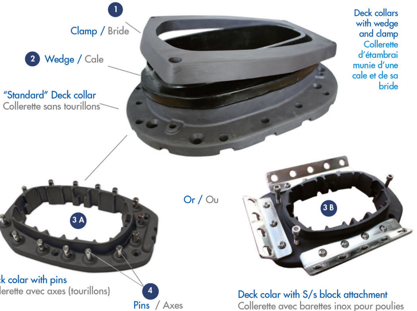
Deck collar including wedging and deck waterproofing, as well as the halyard blocks for keel stepped masts.
